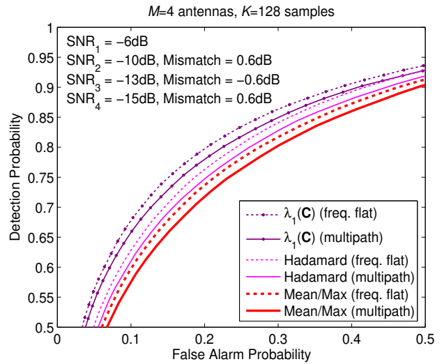
Fig. 7. ROC for the different detectors ( M = 4 ) with noise power mismatch under frequency selective fading.
