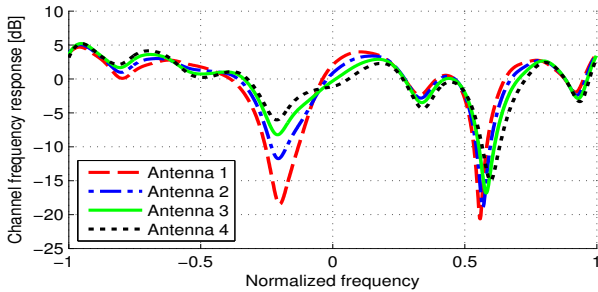
Fig. 6. Channel frequency response in a multipath scenario.
