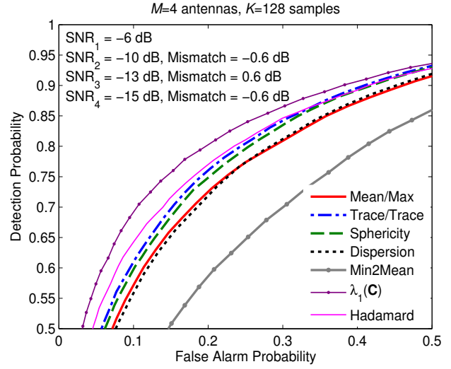
Fig. 4. ROC for the different detectors ( M = 4 ) with noise power mismatch.
