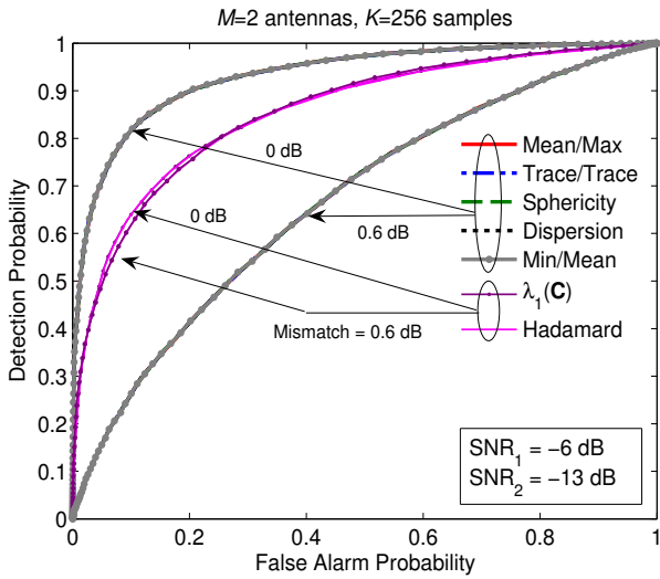
Fig. 1. ROC for the different detectors ( M = 2 ) with and without noise power mismatch.
