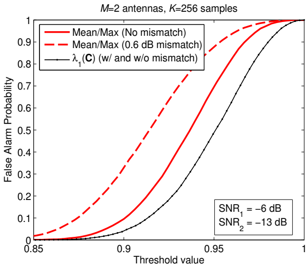
Fig. 2. P_{FA} for the different detectors ( M = 2 ) with and without noise power mismatch.
