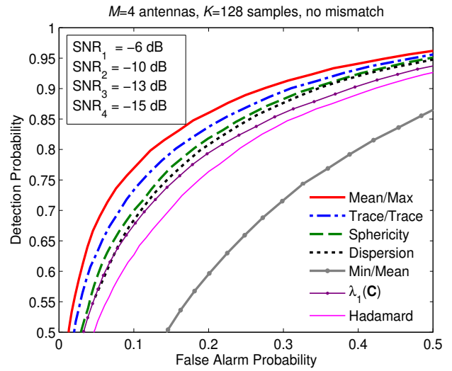
Fig. 3. ROC for the different detectors ( M = 4 ) without noise power mismatch.
