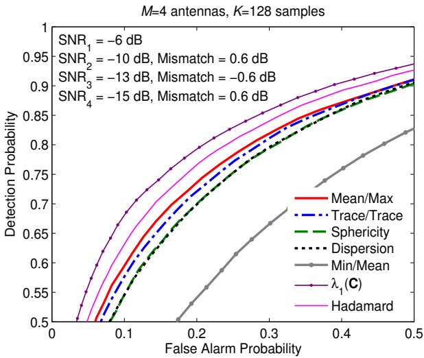
Fig. 5. ROC for the different detectors ( M = 4 ) with noise power mismatch.
